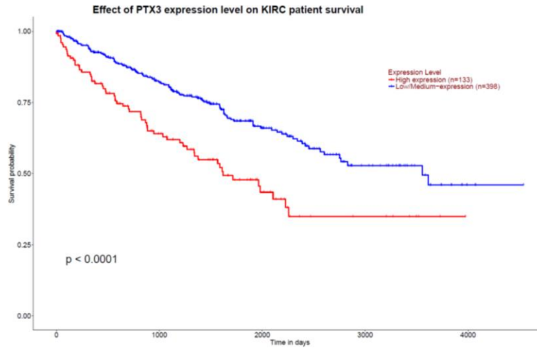
Supplementary Figure 1. Kaplan-Meier survival curves, stratified by the expression level (FPKM) of PTX3 in the tumor tissue at the time of diagnosis. Data from the cancer genome atlas (TCGA) clear cell renal cell carcinoma patient cohort (KIRC).
