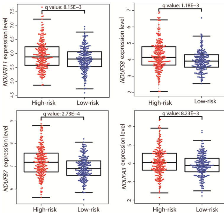
Supplementary Figure 1. Expression differences in the four NADH dehydrogenase genes between the two risk groups. Distribution of NDUFA3 , NDUF7 , NDUF58 , and NDUF11 expression in the two risk groups. The expression levels are represented by log 2 -transformed RPKM values. The P value was calculated by a two-sided Student's t test and adjusted using the Benjamini–Hochberg method.
