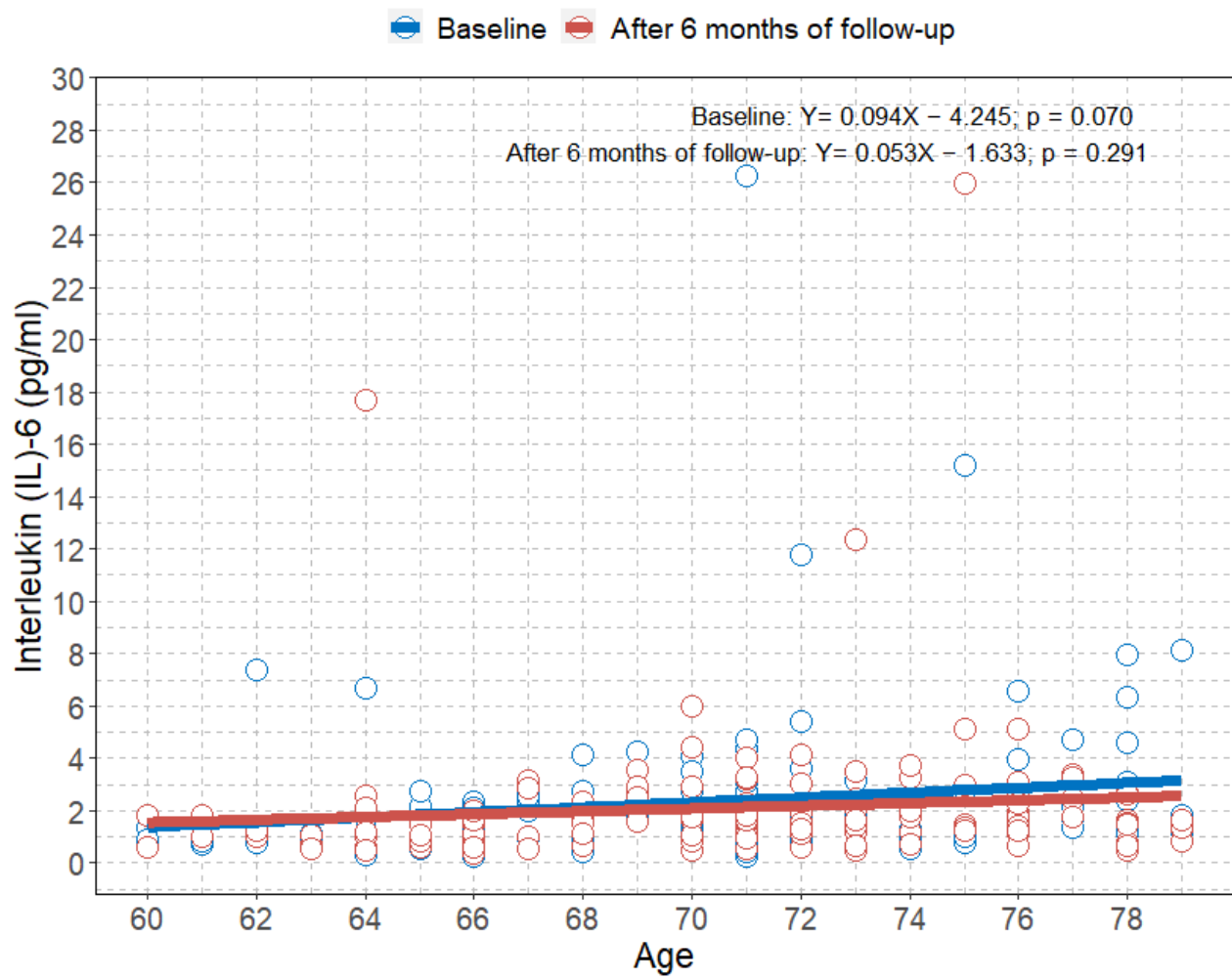
Supplementary Figure 3. Scatterplot with a linear regression line showing the association between age and IL-6 level at baseline and after six months of follow-up. IL-6= interleukin-6.
