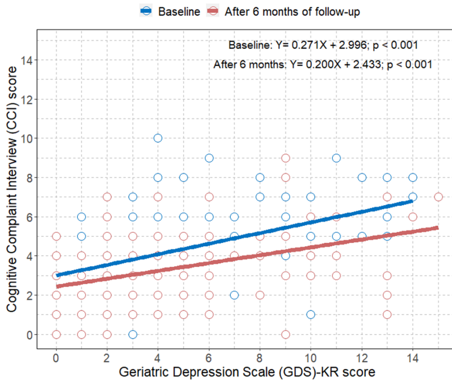
Supplementary Figure 2. Scatterplot with a linear regression line showing the association between the GDS-KR score and CCI at baseline and after six months of follow-up. GDS-KR=Geriatric Depression Scale revised Korean version; CCI=Cognitive Complaint Interview.
