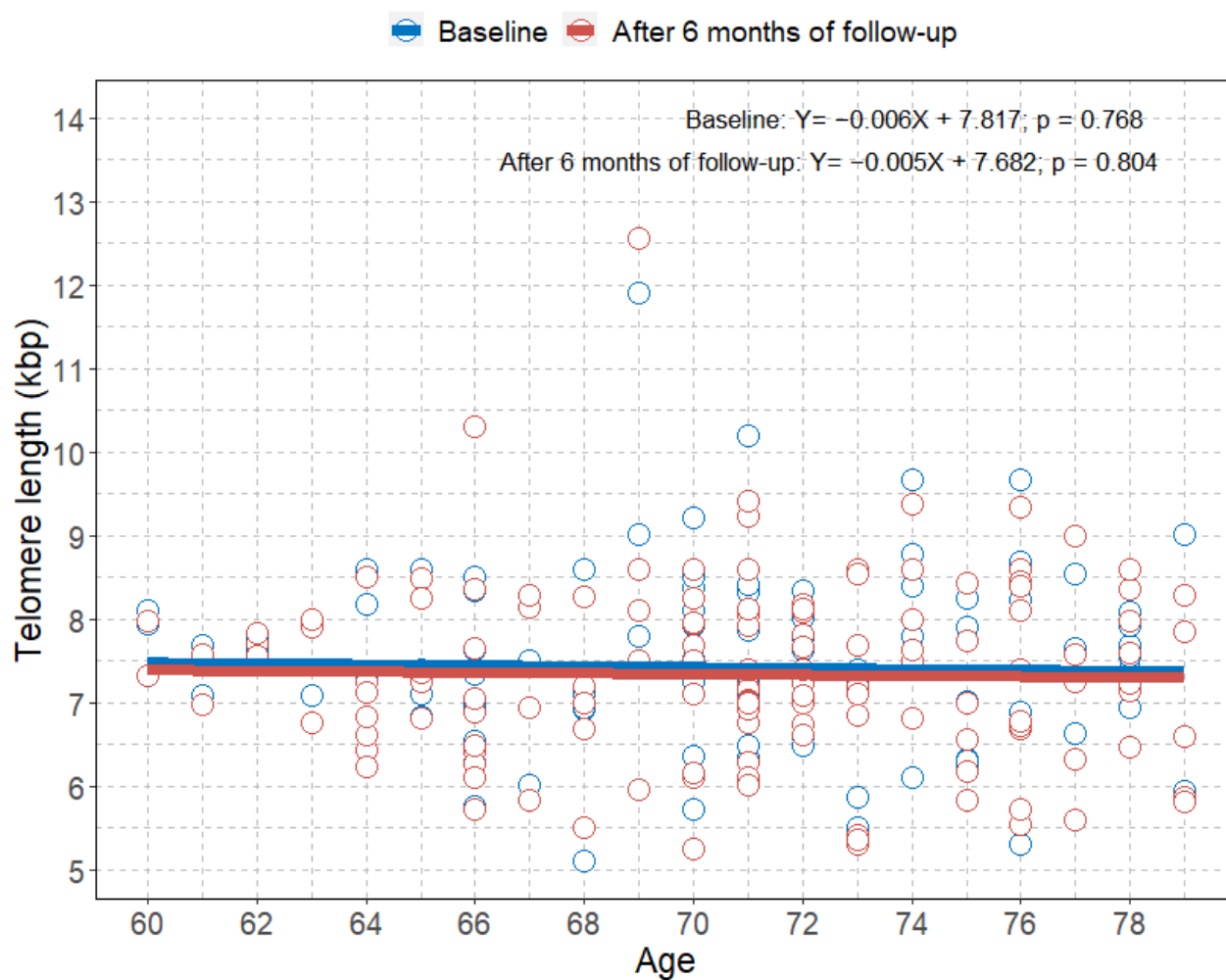
Supplementary Figure 1. Scatterplot with a linear regression line showing the association between age and the TL at baseline and after six months of follow-up. TL=telomere length.
