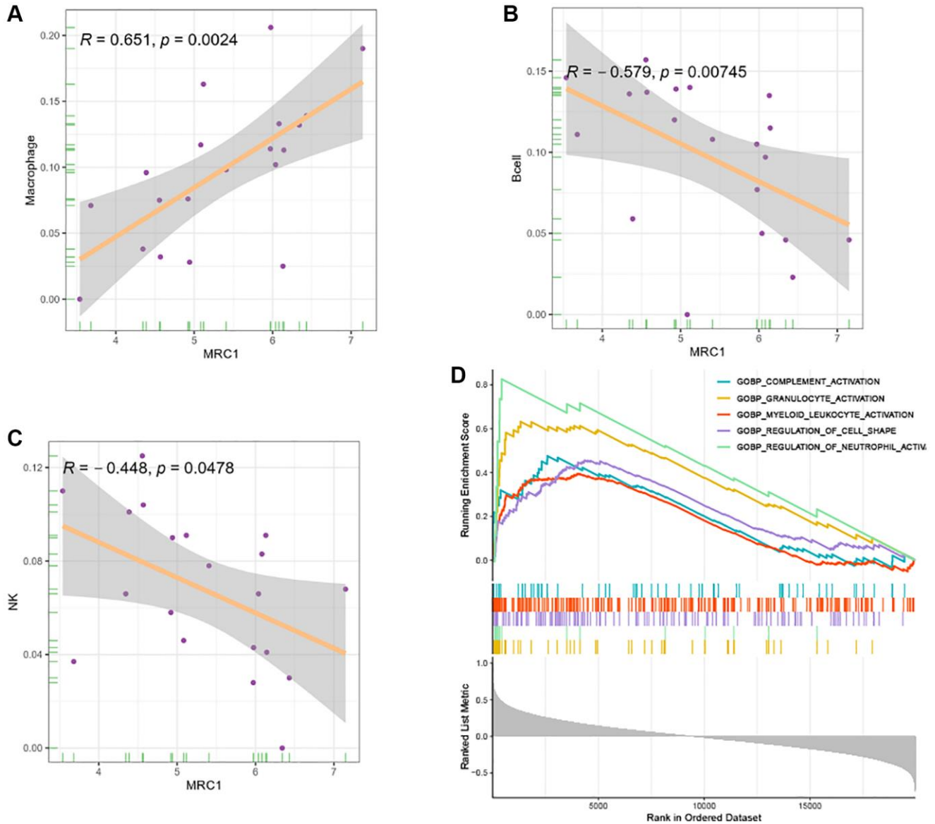
Supplementary Figure 1. Function of MRC1 in SCM. (A) Scatterplot of MRC1 correlation with macrophages. (B) Scatterplot of MRC1 correlation with B cells. (C) Scatterplot of MRC1 correlation with NK cells. (D) Top five GO BP associated with MRC1. Abbreviation: GO: Gene Ontology; BP: biological process; GSEA: Gene Set Enrichment Analysis.
